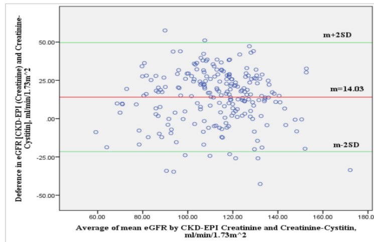
Figure 3: Comparisons of glomerular filtration rate estimated with eGFRCr and eGFRcys-Cr (Bland-Altman test) (n=222)
